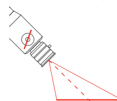
Without tilt adjustment, the pattern features are only partly focused
